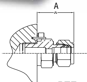
PTFree male connectors (Code FRCM)
